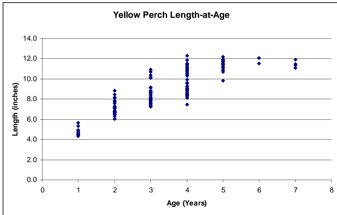
Figure 1. Length at age for Northwest River yellow perch.
