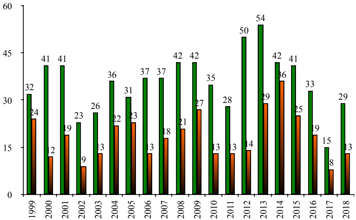
Figure 1. Electrofishing catch rates, fish per hour, for largemouth bass (green columns) and smallmouth bass (orange columns) in South Holston Reservoir 1999-2018.
