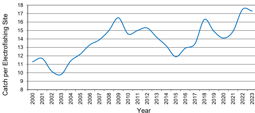
Smith Mountain Lake annual catch rate for Largemouth Bass (≥ 8 inches) collected during DWR sampling each spring.
