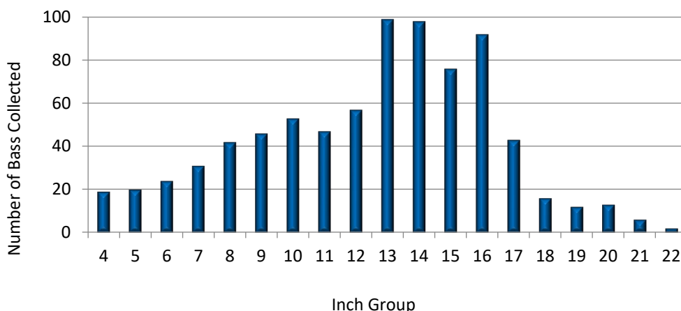
Smith Mountain Lake Largemouth Bass data collected during DWR sampling in the spring of 2023. Each bar represents the number of bass collected for each inch group.
